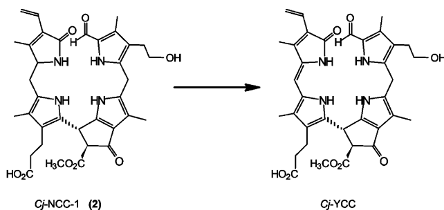
Scheme 6. Oxidation of Cj -NCC-1 ( 2 ) with dicyanodichlorobenzene (DDQ) yields Cj -YCC, a yellow tetrapyrrolic chlorophyll catabolite. [52]
