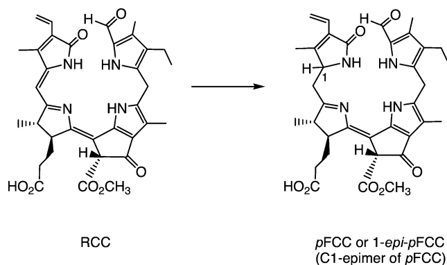
Scheme 2. Two stereodivergent lines of RCC reductases occur in (senescent) higher plants, each giving one of two epimeric ‘primary’ FCCs ( p FCCs) by stereoselective reduction of (enzyme-bound) red chlorophyll catabolite (RCC). [26,27]
