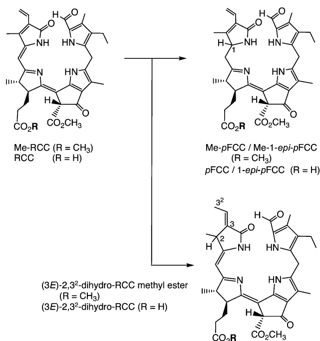
Scheme 4. Electrochemical reduction of red chlorophyll catabolite (RCC) or of its methyl ester (Me-RCC) leads to the two epimeric primary FCCs ( p FCC and epi - p FCC) or their methyl esters, respectively, as well as to regioisomeric 2,3 2 -dihydro-RCCs and their methyl esters. [41,42]
